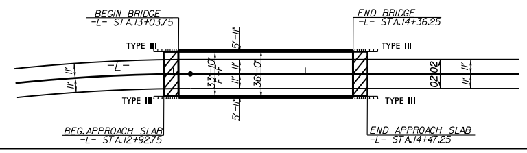
SKETCH SHOWING BRIDGE/PAVEMENT RELATIONSHIP
